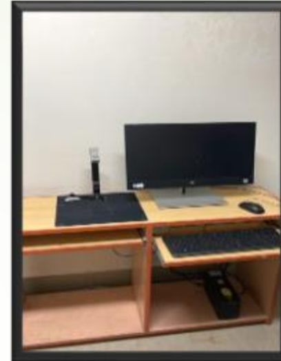
Braille Software
